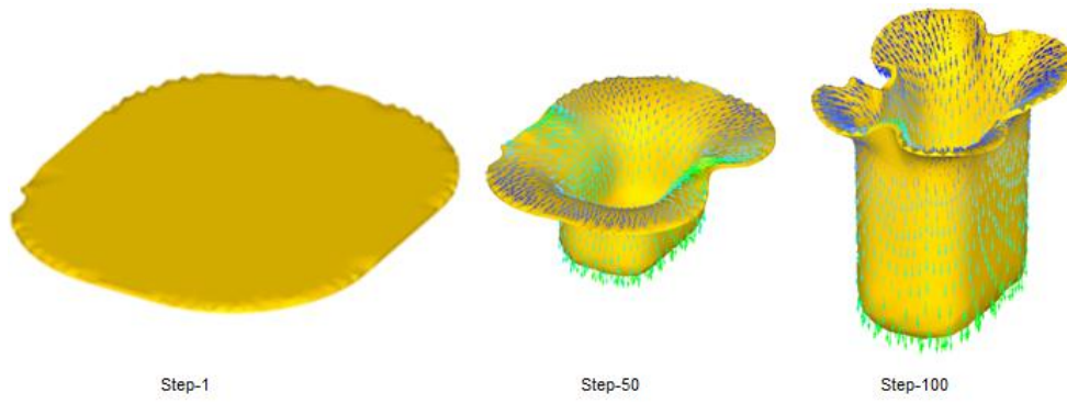
Figure 3: Rectangular cup drawing at different steps.
