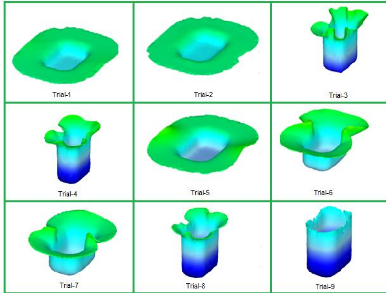
Figure 7: Heights of rectangular cups under different operating conditions.
