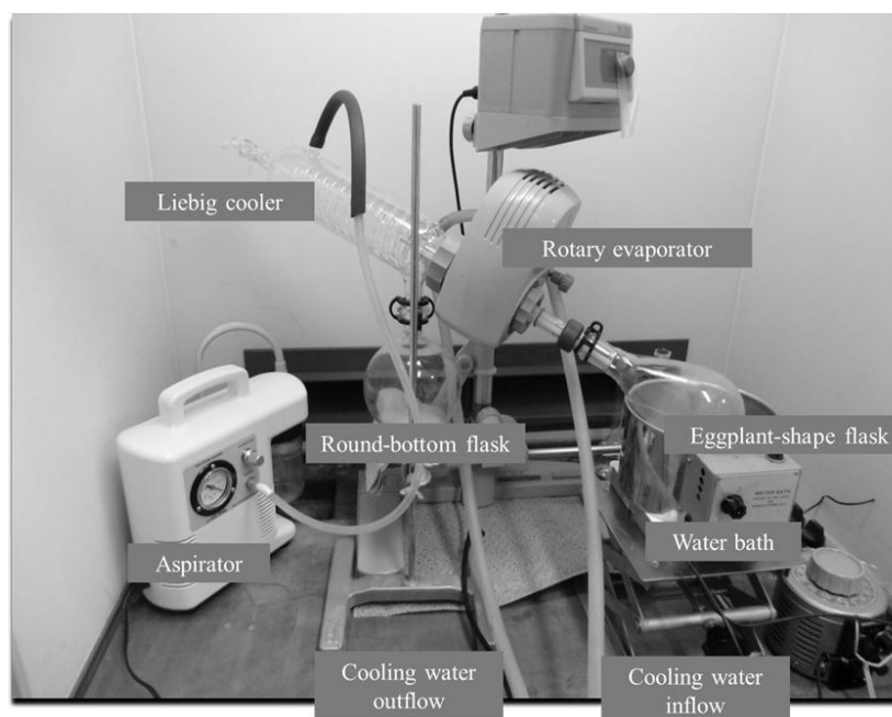
Figure 1:- The apparatus setting of vacuum distillation
