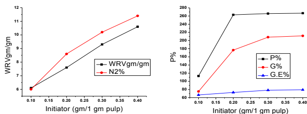
Effect of initiator concentration sample B
