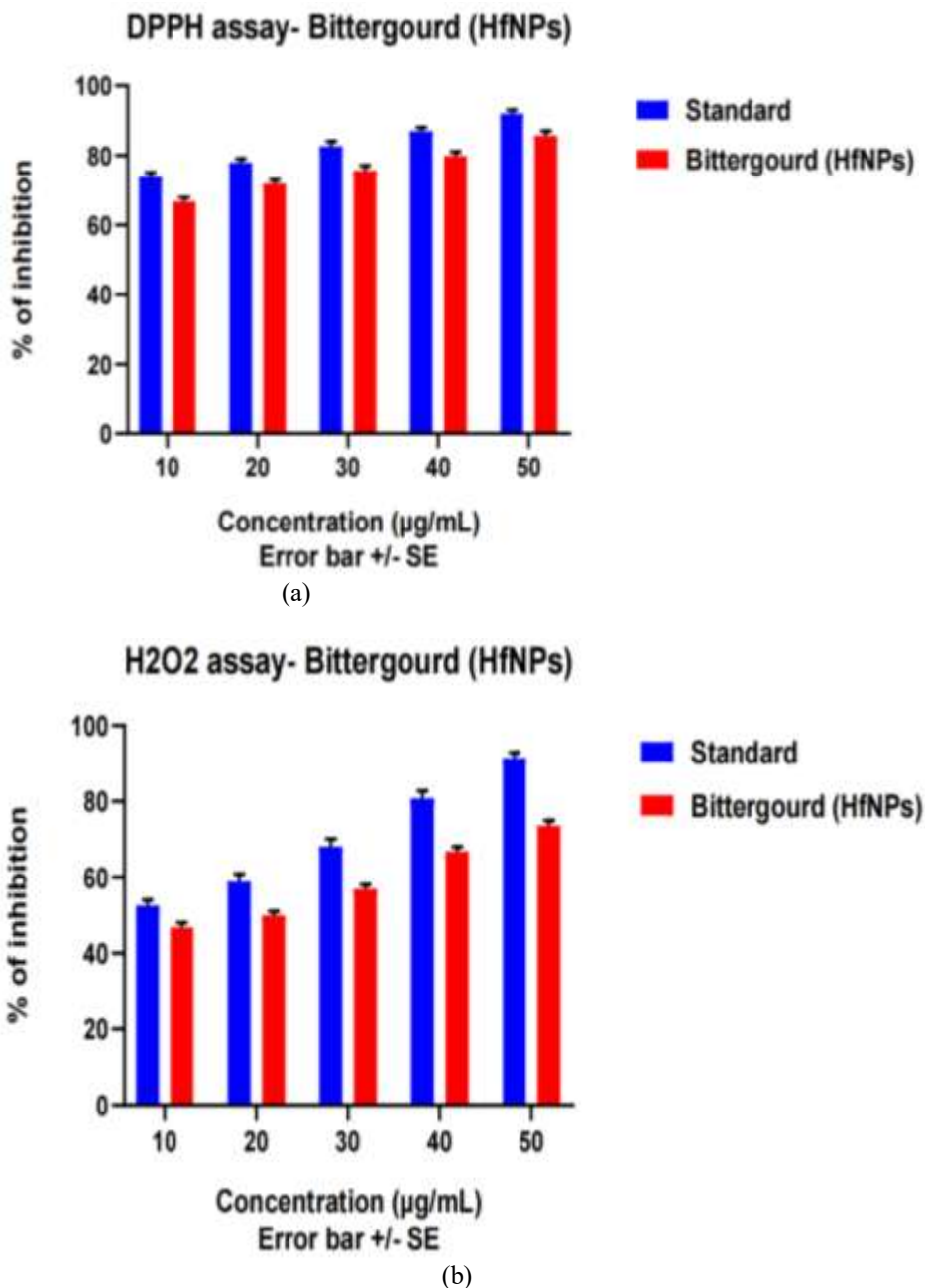
Figure 3:- Estimation of Antioxidant activity of Momordica Charantia synthesized Hafnium oxide Nanoparticles using (a) DPPH assay , (b) Hydrogen peroxide assay.
