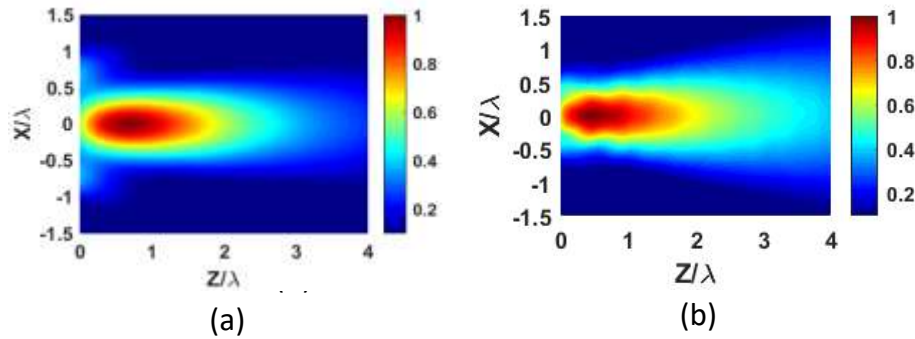
Fig.6:- Mapping of the normalized transverse electric field intensity in the plane defined by the propagation direction ( z ) and the vertical polarization of the excitation ( x ): (a) simulated mapping and (b) Measured mapping.
