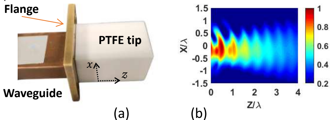
Fig. 3:- (a) 3D view of Prototype No. 1, illustrating the waveguide equipped with a flange terminated by a PTFE tip. (b) Measurements of the normalized electric field intensity distribution ( |E|^2 ) in free space at the output of the rectangular waveguide with a PTFE extension, for a frequency of 15 GHz.
