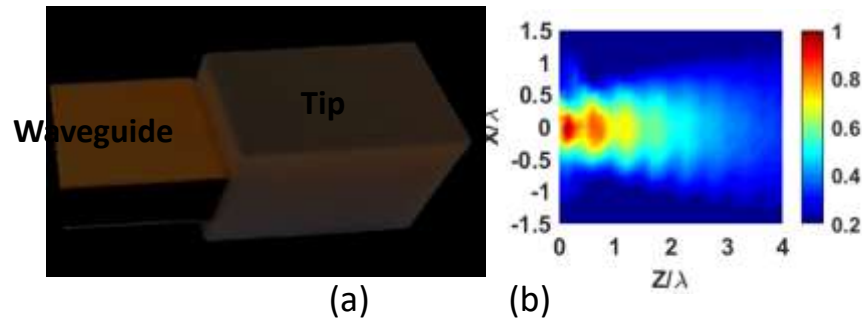
Fig. 4:- (a) 3D view of Prototype No. 2 illustrating the waveguide without a flange, terminated by a PTFE tip. (b) Measurements of the normalized electric field intensity distribution ( |E|^2 ) in free space at the output of the rectangular waveguide with a PTFE extension, for a frequency of 15 GHz.
