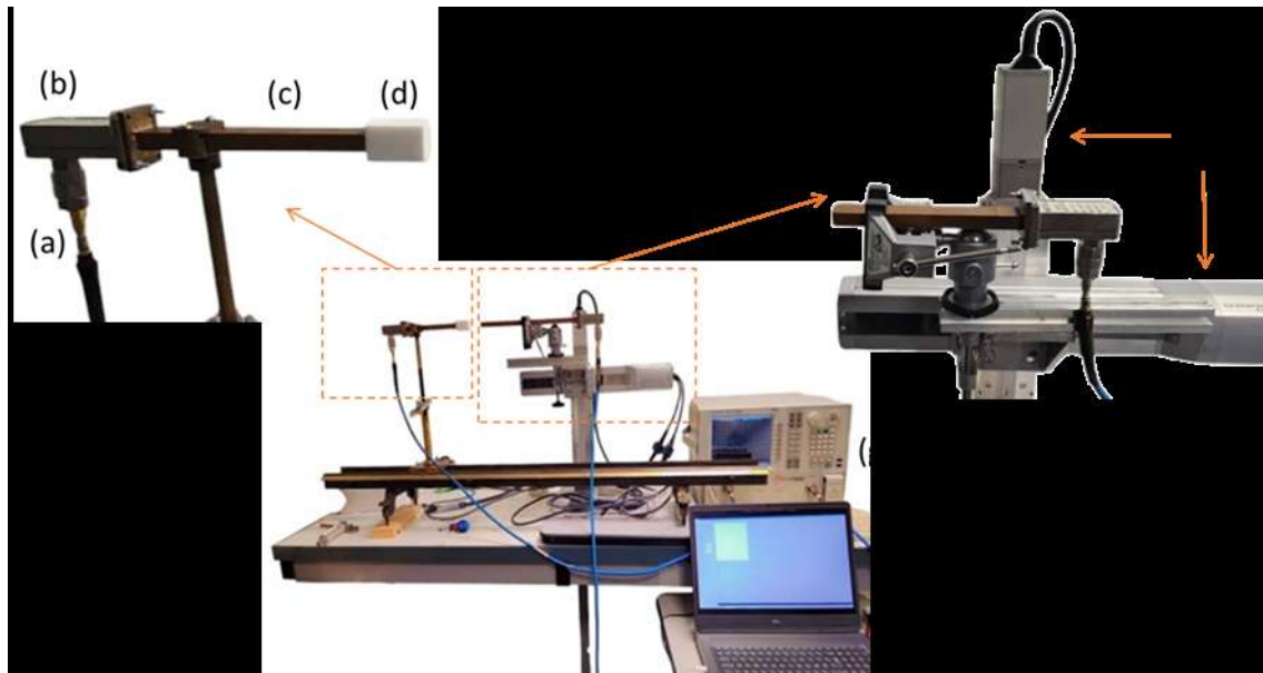
Fig. 2:- Experimental setup for mapping the electromagnetic field generated at the end of the PTFE extension of the rectangular waveguide. (a) coaxial cable (b) WR/Coaxial transition (c) rectangular waveguide (d) PTFE tip (e) open rectangular guide probe (f) two-axis robotic arm (g) VNA (h) Control PC.
