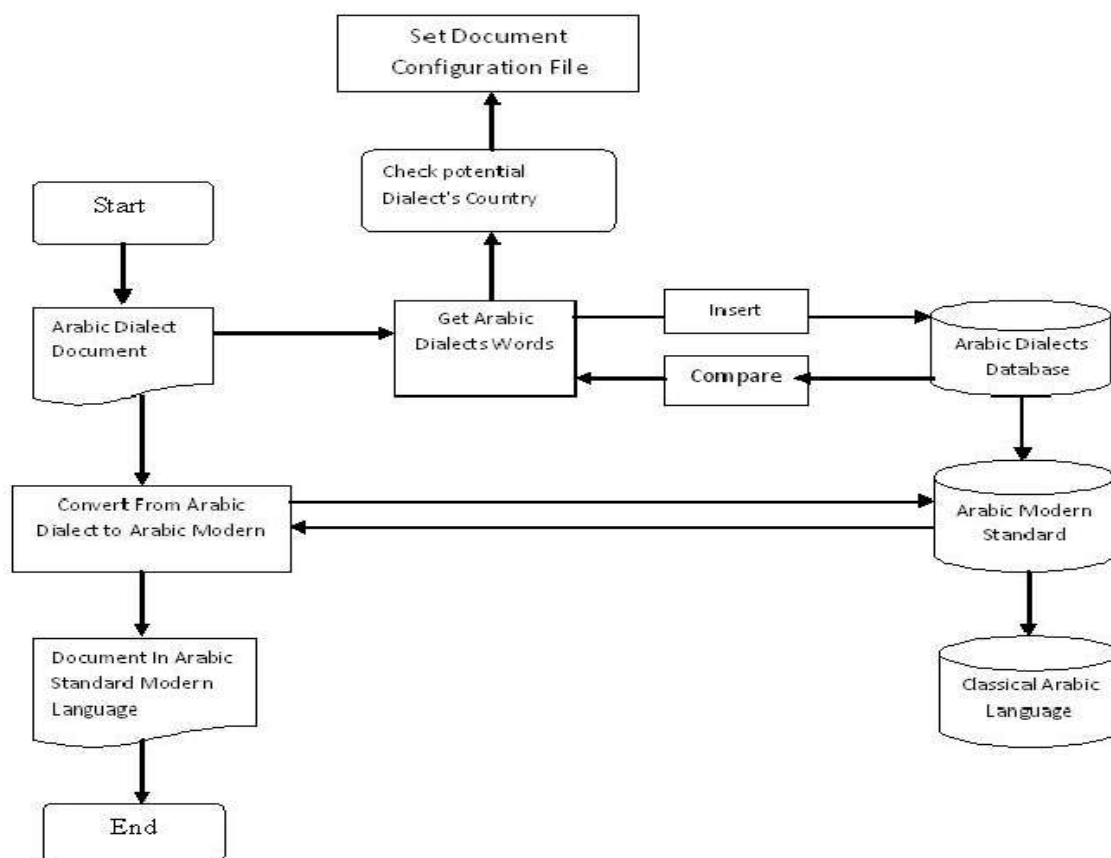
Figure 3:- Building new Lexicon of Libyan dialects.
