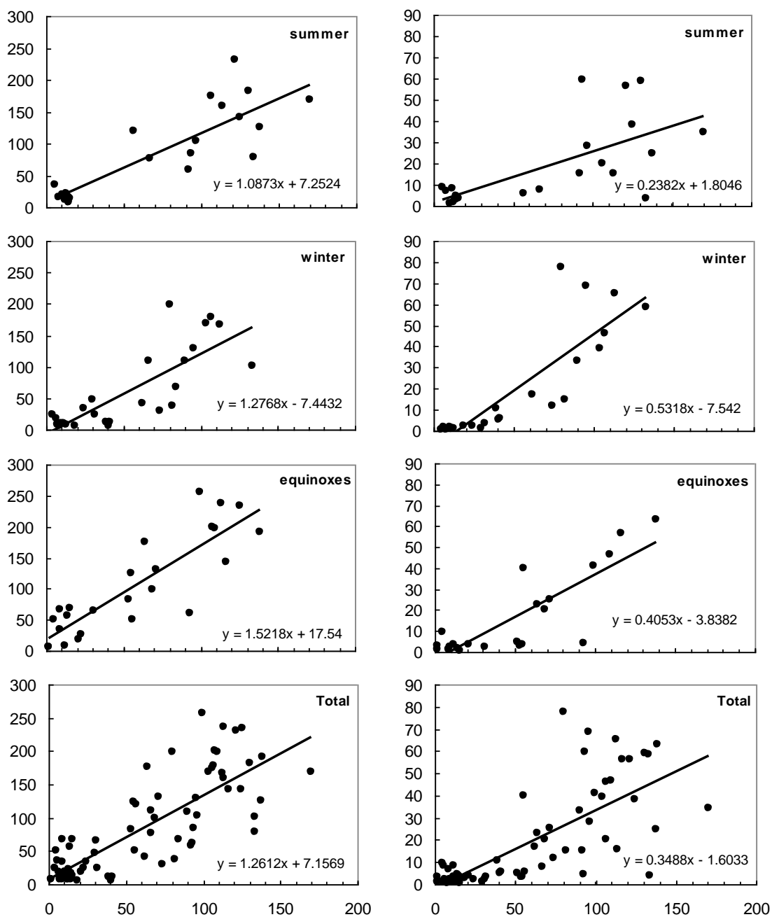
Figure 4: Variation of average daytime (left column) and nighttime (right column) electron density observed by the SROSS C2 satellite with R_z within \pm 10^\circ magnetic latitude.
