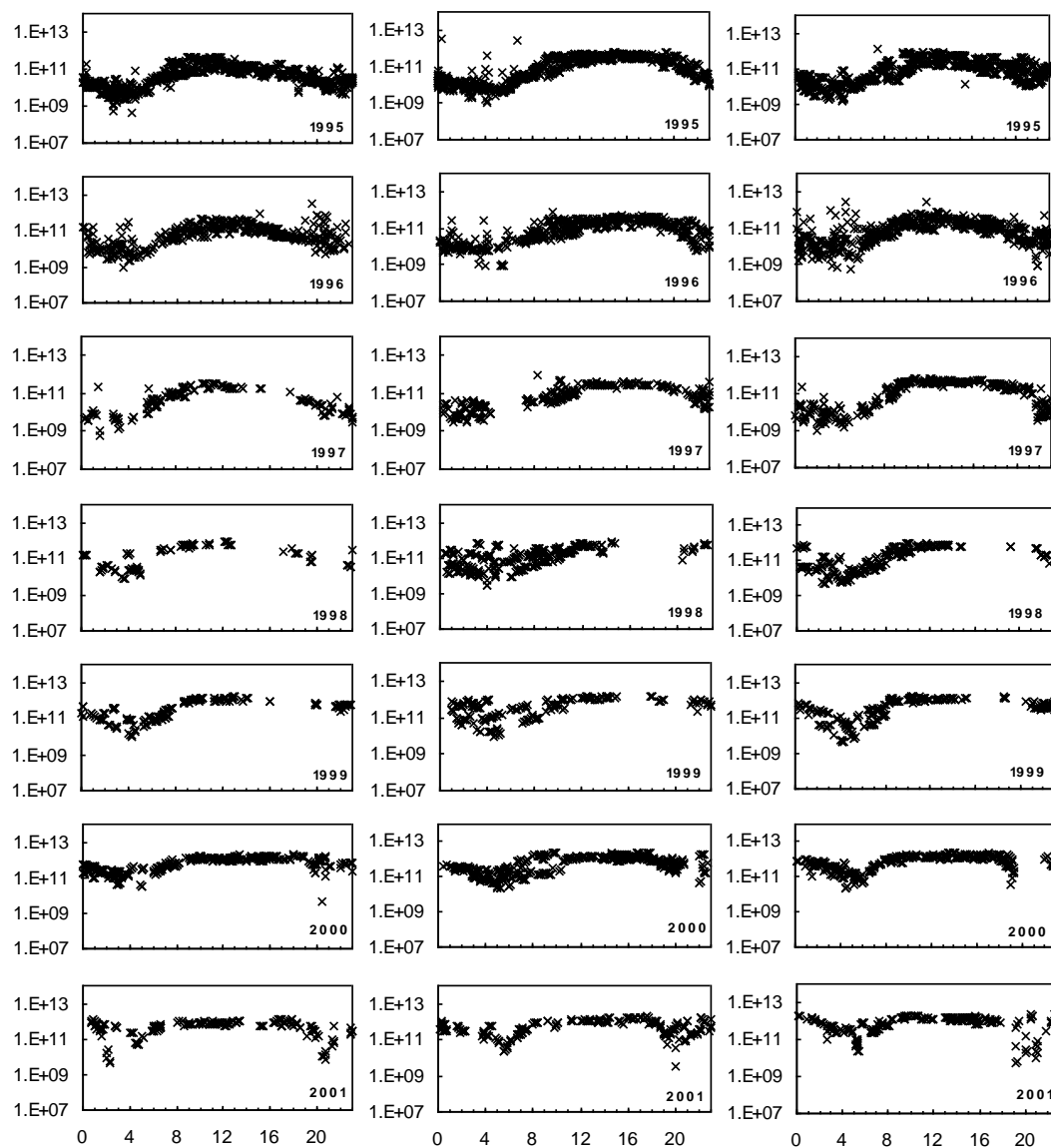
Figure 2: Local time and seasonal variation of electron density measured by the SROSS C2 at the altitude of \sim 500 km within \pm 2.5^\circ of the geomagnetic equator for the years 1995 to 2001.
