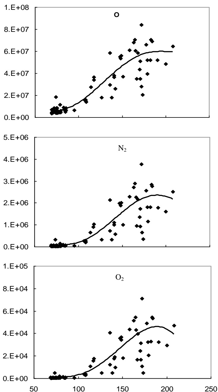
Figure 8: Scatter plot of neutral density of O, N 2 and O 2 against corresponding solar flux from the MSIS-86 model. The solid line in each block represents the 5 th order polynomial fit to the data.
