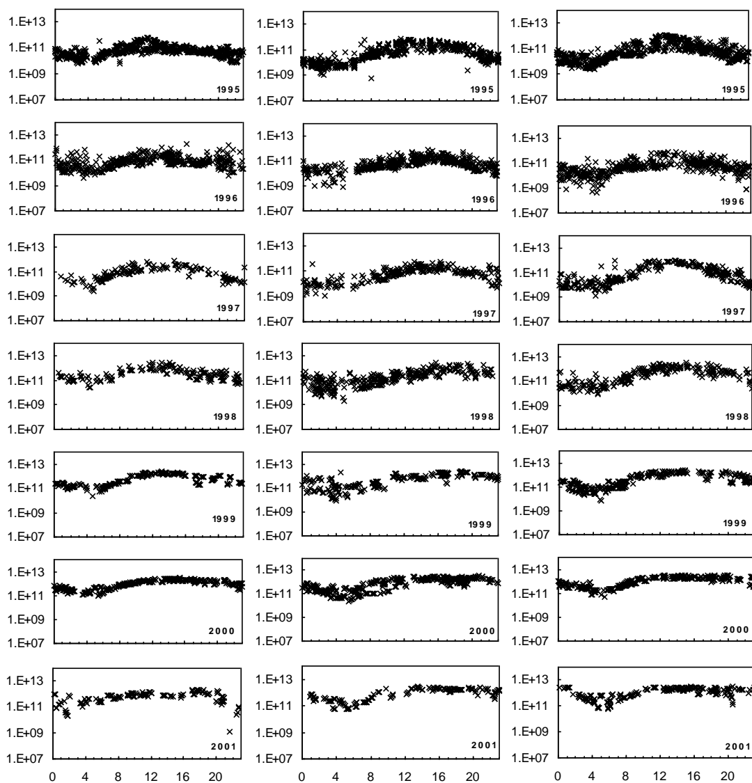
Figure 1: Diurnal and seasonal variation of electron density measured by the SROSS C2 at the altitude of \sim 500 km over 10^\circ \pm 2.5^\circ N magnetic latitude for the years 1995 to 2001.
