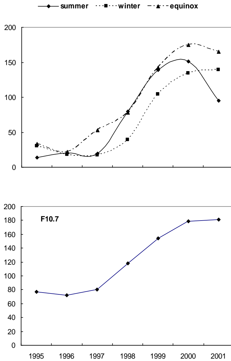
Figure 6: Variation of mean annual daytime (10:00 – 14:00 hr LT) electron density and F10.7 averaged for each year of observation from 1995 to 2001.
