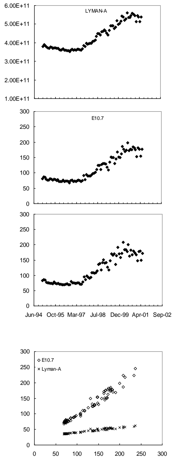
Figure 7: Month to month variation of Lyman- \alpha , E10.7 and F10.7 during the period January 1995 to June 2001. The figure also shows plots of Lyman \alpha and E10.7 against F10.7 cm flux.
