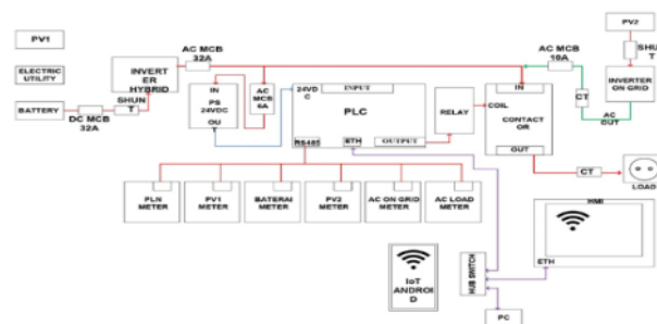
Figure 6. Block Diagram of Battery to PLC Mode
