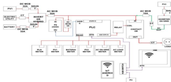
Figure 4. Block Diagram of Total Control System Technology (TCST)
