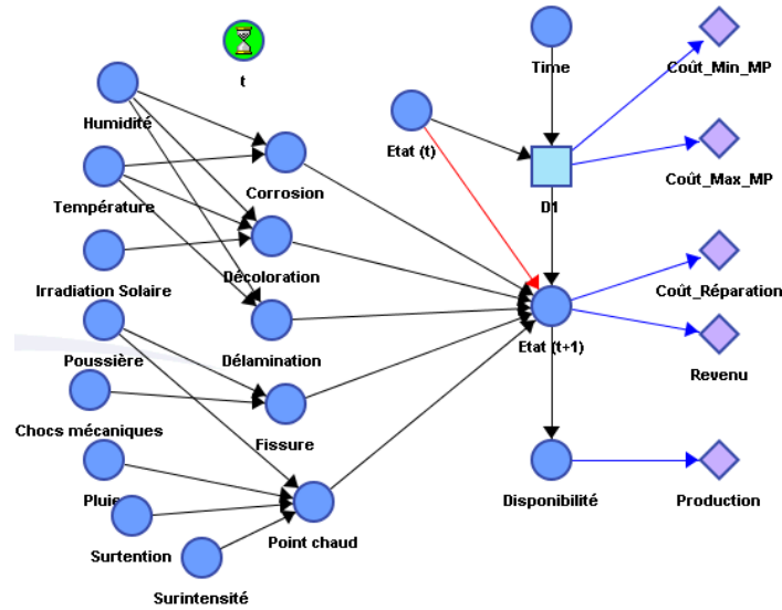
Figure 13: Bayesian multi-state model with performance indicators
