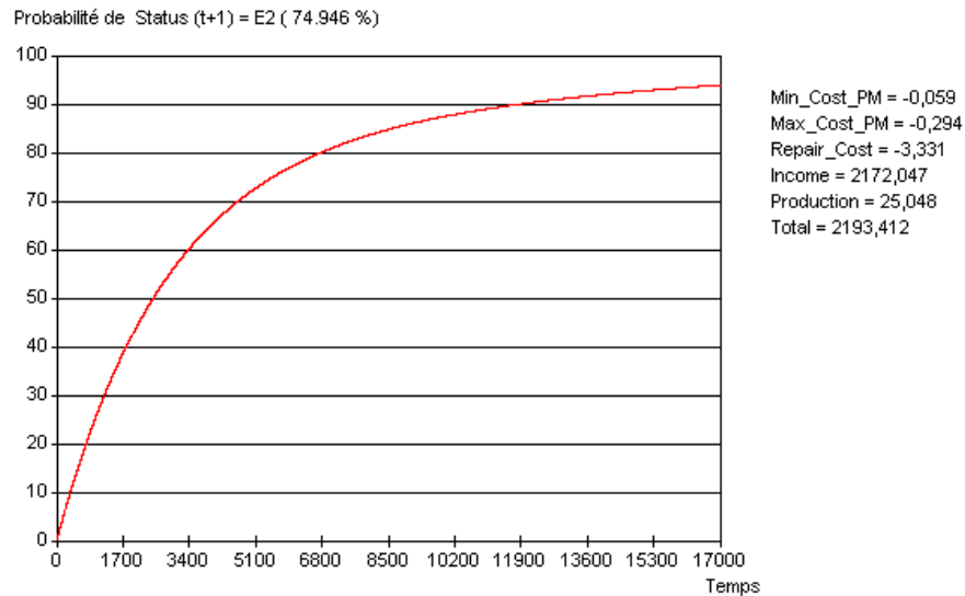
Figure 7: The evolution of the degradation process of E_2
