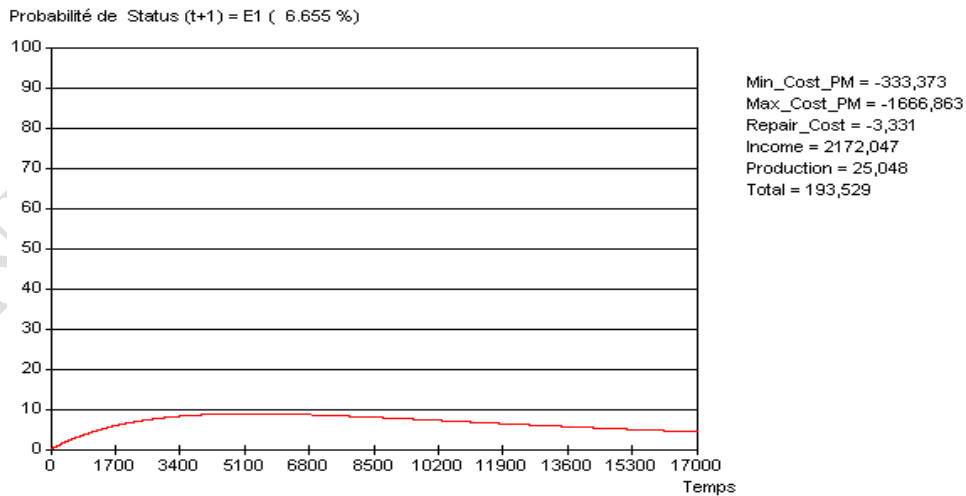
Figure 6: Evolution of the E_1 degradation process
