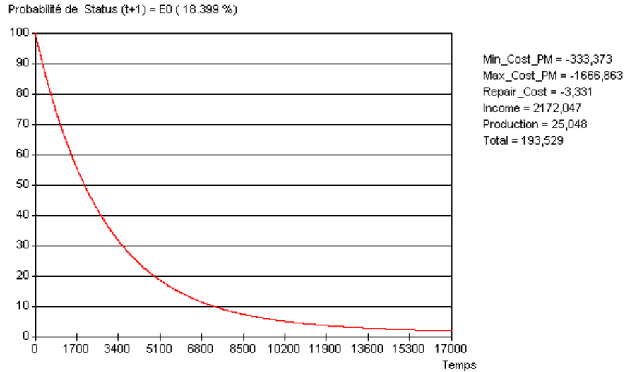
Figure 5: Evolution of the E_0 degradation process
