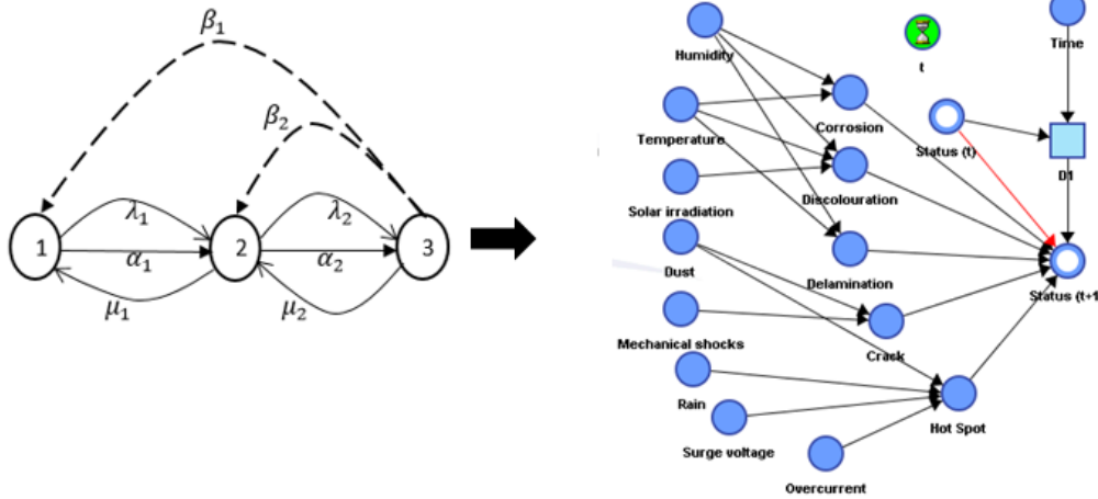
Figure 1: Markov model to PV module dynamic degradation Bayesian model
